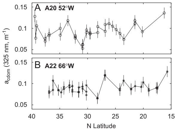
Fig. 7. Distribution of CDOM (as 325 nm absorption coefficient, m^{-1} ) within the subtropical mode water (defined as neutral density interval between 26.4 and 26.6 kg\ m^{-3} ) along the A20 line, 52°W (A) and the A22 line, 66°W (B). Error bars are the 95% confidence interval for a single estimate (see Methods).
