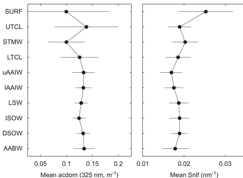
Fig. 9. Mean CDOM absorption coefficients (325 nm, m -1 ) for samples collected within each layer (cf. Table 1). Error bars are the standard deviation.
