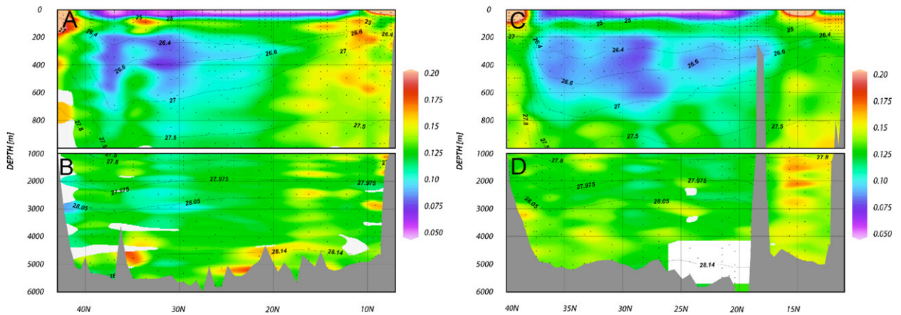
Fig. 6. Distribution of CDOM (as 325 nm absorption coefficient, m^{-1} ) along 52°W (A20 section, (A) and (B)) and 66°W (A22 section, (C) and (D)), as in Fig. 3.
